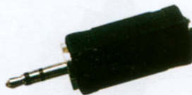
FC-A-0708 (4007,4008) 4007:2.5mm STEREO plug to 3.5mm STEREO jack adaptor 4008:2.5mm STEREO plug to 3.5mm MONO jack adaptor
