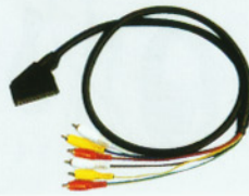
FC-A-0456 (8030J93) SCART female to 6xRCA male audio in & out video in & out O.D.9mm round cable
