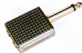
FC-A-0787 (4082HQQ,4082N) 4082HQQ:GOLD 6.3mm MONO plug to 2x3.5mm MONO jack adaptor 4082N:nickel 6.3mm MONO plug to 2x3.5mm MONO jack adaptor
