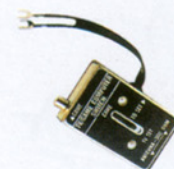
FC-A-1061 (5121) TV game computer switch I/P -1RCA jack 75Ω/300Ω O/P -300Ω
