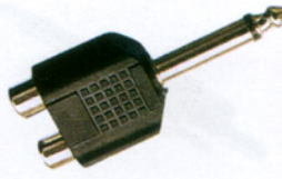
FC-A-0765 (4064) 6.35mm MONO plug to 2xRCA jack adaptor
