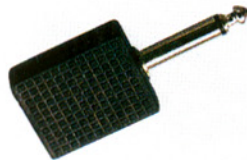
FC-A-0786 (4082,4083) 4082:6.35mm MONO plug to 2x3.5mm MONO jack adaptor 4083:6.3mm MONO plug to 2x3.5mm STEREO jack adaptor
