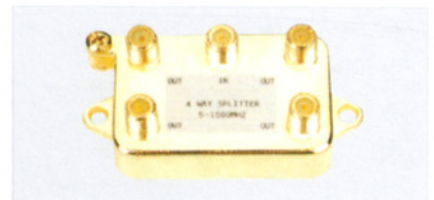
FC-A-1067 (G303) 4-way splitter 5-1000 MHz
