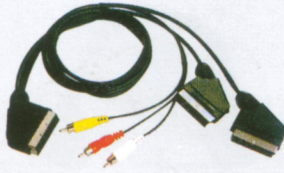
FC-A-0353 (8016H) SCART male to 2xSCART male +3xRCA male electronic cable O.D.5+2.6x7.8mm
