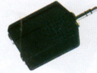
FC-A-0781 (4078,4079) 4078:3.5mm STEREO plug to 2x6.3mm STEREO jack adaptor 4079:3.5mm STEREO plug to 2x6.3mm MONO jack adaptor
