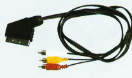
FC-A-0402 (8023) SCART male to 3xRCA male audio/video in flat cable
