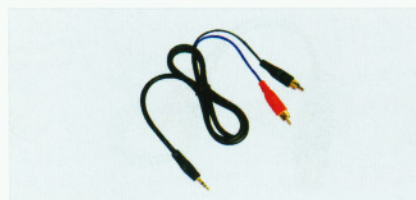
FC-A-0053 (8057H) 3.5mm STEREO male to 2xRCA male O.D. 5.0mm cable
