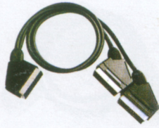
FC-A-0350 (8016D,8016D54,8016D61,8016DS60) 8016D:SCART male to 2xSCART male 8C+1 electronic cable 8016D54:SCART male to 2xSCART male O.D.5mm 6C+1 electronic cable 8016D61:SCART male to 2xSCART male O.D.6mm 6C+1 electronic cable 8016DS60:SCART male to SCART male /out +SCART male /in O.D.6mm electronic cable
