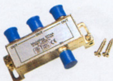
FC-A-1044 (5109A,5109B) 5109A:3-way splitter 5-1000 MHz 5109B:3-way splitter 5-2050 MHz
