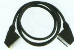
FC-A-0337 (8017B,8017BX,8017BG) 8017B: SCART male to SCART male 20C+1 standard cable 8017BX: SCART male to SCART male 20C+1 standard cable cross connection 17-18 18-17 8017BG: GOLD SCART male to SCART male 20C+1 standard cable
