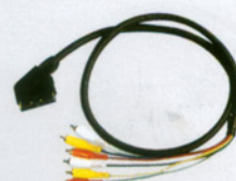
FC-A-0454 (803093) SCART male to 6xRCA male audio in & out video in & out O.D.9mm round cable
