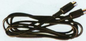
FC-A-0035 (8042,8042A,804253) 8042:DIN 5pin male to DIN 5pin male O.D.5.0mm cable 8042A:DIN 5pin male to DIN 5pin female O.D.5.0mm cable 804253:DIN 5pin male to DIN 5pin male O.D.5.0mm cable 4-4 5-5 G/2-2
