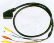
FC-A-0440 (802673) SCART male to 4xRCA male audio in & out jump wire video in & out O.D.7mm round cable
