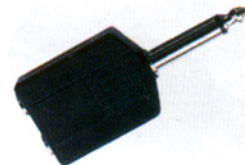
FC-A-0790 (4086,4087) 4086:6.35mm MONO plug to 2x6.35mm MONO jack adaptor 4087:6.35mm MONO plug to 2x6.35mm STEREO jack adaptor
