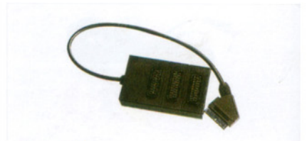
FC-A-0322 (8007,8007M,800781) 8007:SCART male to 3xSCART female W/cable 8007M:SCART male to 3xSCART female W/cable mini type 800781:SCART male to 3xSCART female solder type O.D.8mm cable
