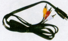
FC-A-0080 (8044J) DIN 6pin female to 3xRCA male O.D.2.6x5.2mm cable
