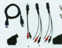
FC-A-0469 (8129A) 1PC DIN 6PIN male-DIN 6PIN male 2m/1PC DIN 5PIN male-2RCA female 0.15m/1PC DIN 6PIN female-3RCA male A/V cable 0.15m (IN)/1PC DIN 6PIN female 3-RCA male A/V cable 0.15m(OUT) 1PC SCART-DIN 6PIN IN/1PC SCART-DIN 6PIN OUT/2PC BNC plug -RCA jack
