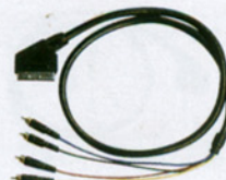
FC-A-0439 (802672) SCART male to 4xRCA male audio in & out jump wire video in & out O.D.7mm round cable
