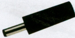
FC-A-0647 (1025A, 1025B, 1025C) 1025A: 2.5x0.7mm DC plug 1025B: 4x1.7mm DC plug 1025C: 3.5x1.4mm DC plug
