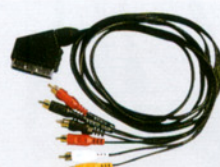
FC-A-0450 (8029) SCART male to 6xRCA male audio in & out video in & out flat cable
