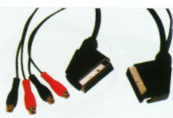
FC-A-0366 (8020EJ) SCART male to SCART male +4RCA female audio/video electronic SCART cable+O.D.2.6x10.4mm cable
