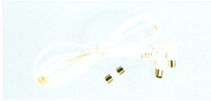
FC-A-0181 (8070) 9.0mm male angle to 9.0mm male angle COAXIAL cable W/9.0 mm(F-F) inline connector
