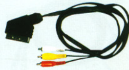
FC-A-0411 (802432) SCART male to 3xRCA male audio/video out flat cable
