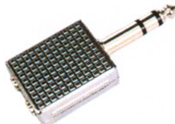
FC-A-0789 (4084HQQ,4084N) 4084HQQ:GOLD 6.3mm STEREO plug to 2x3.5mm STEREO jack adaptor 4084N:nickel 6.3mm STEREO plug to 2x3.5mm STEREO jack adaptor
