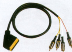
FC-A-0441 (8026MPG) GOLD SCART male to 4xRCA male audio in & out jump wire video in & out round cable
