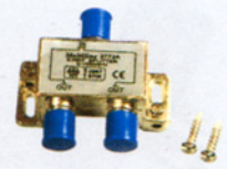
FC-A-1043 (5018A,5018B) 5018A:2-way splitter 5-1000 MHz 5018B:2-way splitter 5-2050 MHz
