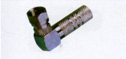
FC-A-0902 (5058L/47,5058L/57,5058L/67) 5058L/47:angle F plug for RG58 cable I.D.4.7mm twist on type 5058L/57:angle F plug for RG59 cable I.D.5.7mm twist on type 5058L/67:angle F plug for RG6 cable I.D.6.7mm twist on type
