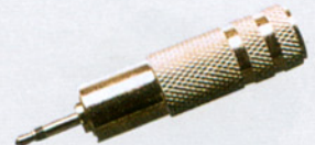
FC-A-0712 (4015,4016) 4015:2.5mm MONO plug to 6.3mm MONO jack metal adaptor 4016:2.5mm MONO plug to 6.3mm STEREO jack metal adaptor
