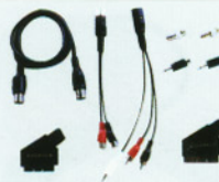
FC-A-0468 (8129) 1PCS DIN 6PIN male-DIN 6PIN male 2M/1PC DIN 5PIN male - 2RCA female 0.15m/1PC DIN 6PIN female-3RCA male A/V cable 0.15m/1PC SCART-DIN 6PIN in/1PC SCART-DIN 6PIN out/2PC BNC plug-RCA jack/2PCS 3.5mm MONO plug-RCA jack
