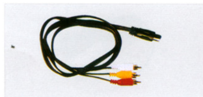
FC-A-0071 (8044) DIN 5pin male to 3xRCA male A/V cable
