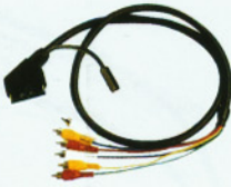
FC-A-0458 (8030MO) SCART male to 6xRCA male audio in & out video in & out video in & out +3.5mm MONO jack round cable
