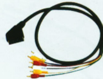
FC-A-0463 (8030R) SCART male to 6xRCA male audio in & out video in & out round cable
